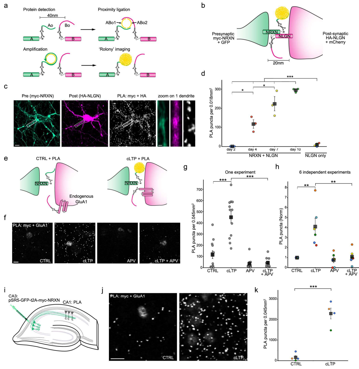
Figure 1: SYNPLA detects synapse formation and potentiation in cultured neurons and slices
